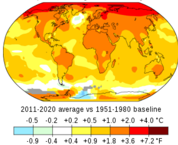
Temperature change in the last 50 years
